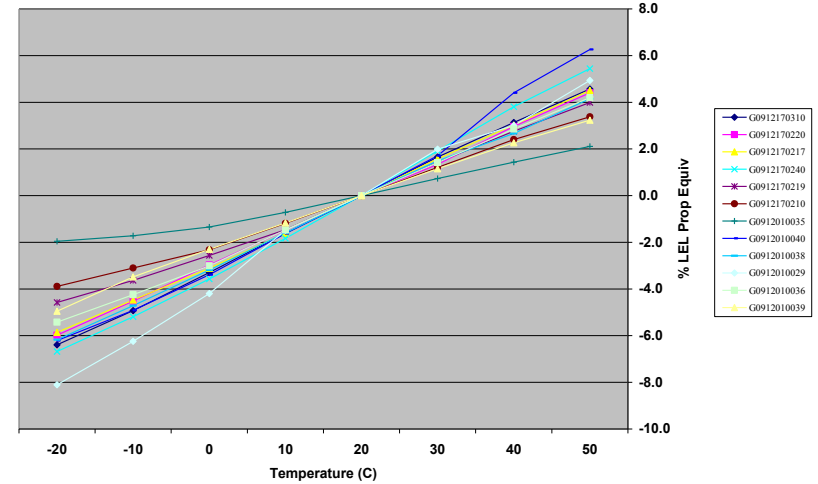
GS-701 G series - Baseline vs Temp (Detector Displayed Zero, Scale - %LEL Propane Equiv) 3-15-2010
